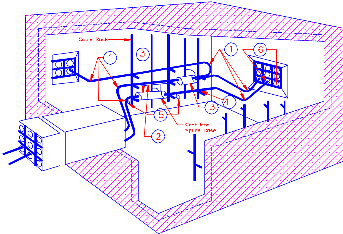
FIGURE 4 UCV UNDERGROUND CABLE AND SPLICE CASE RACKING DIAGRAM EXAMPLE
