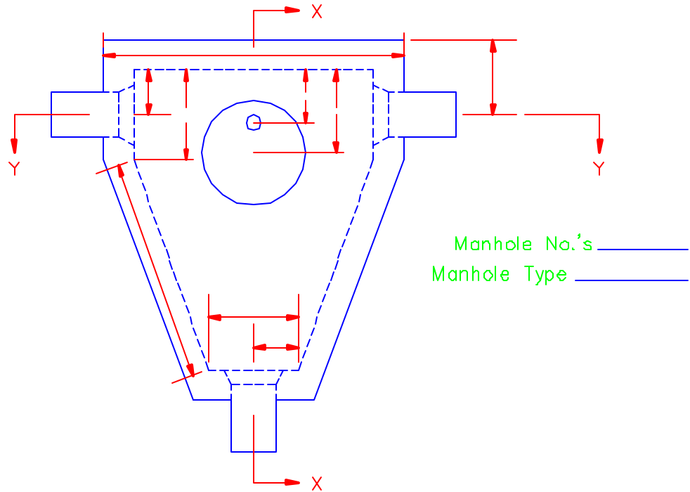
FIGURE 2 EXAMPLE OF CONSTRUCTION DETAILS POURED-IN-PLACE UCV TYPE V
