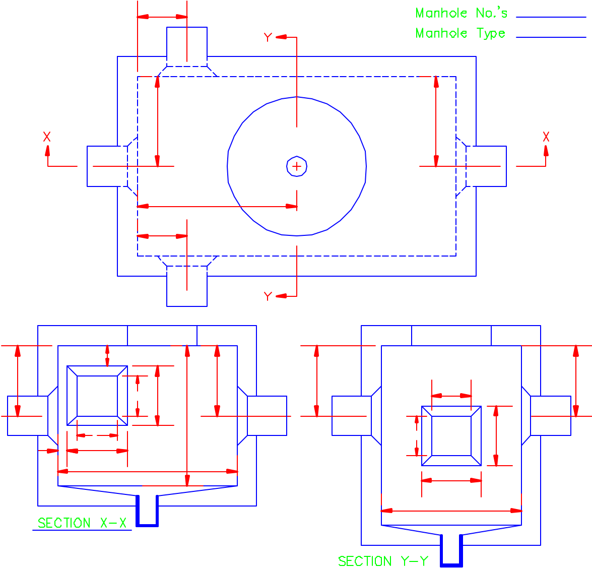
FIGURE 1 EXAMPLE OF CONSTRUCTION DETAILS POURED-IN-PLACE UCV TYPES A, L, T, J, X, AND Y
