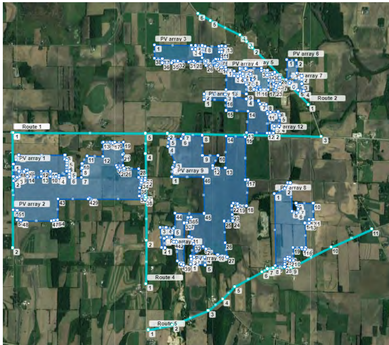
Figure 1: Badger Solar Project PV Array approximate Layout in ForgeSolar, including vehicle routes on roadways adjacent to the Project.
